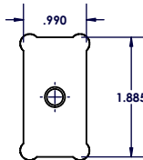
VF1+8-CP 8MM MACHINABLE
